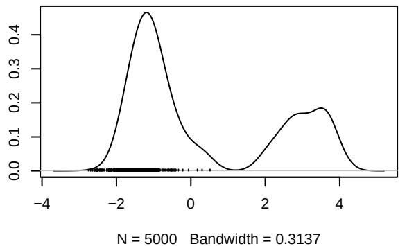
Density of b[2]
