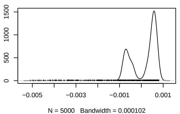
Density of b[3]
