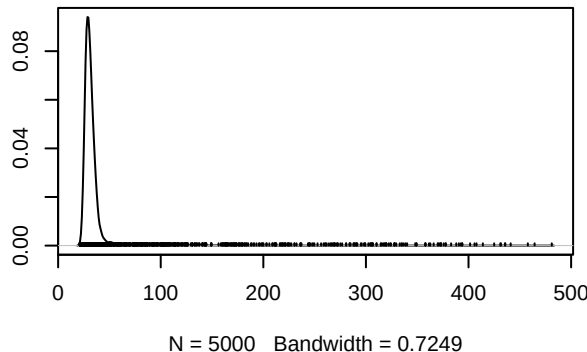
Density of \text{sig}
