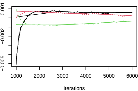
Trace of b[3]
